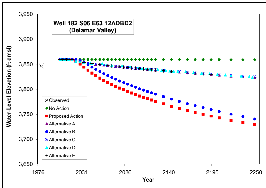
Figure 3.3.2-8 Representative Water-Level Hydrograph for Cave, Dry Lake, and Delamar Valleys
